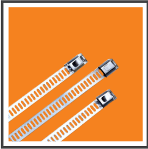
Type: Ladder Type Un-coated Width: 7 mm and 12 mm Material: SS 304 & SS 316
